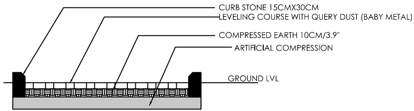
PATHWAY DETAIL C-C WIDTH = 200CM
