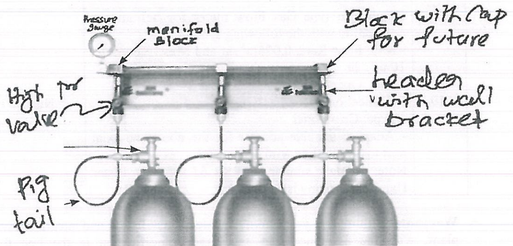
Wall Mounted Helium Valve Manifold
