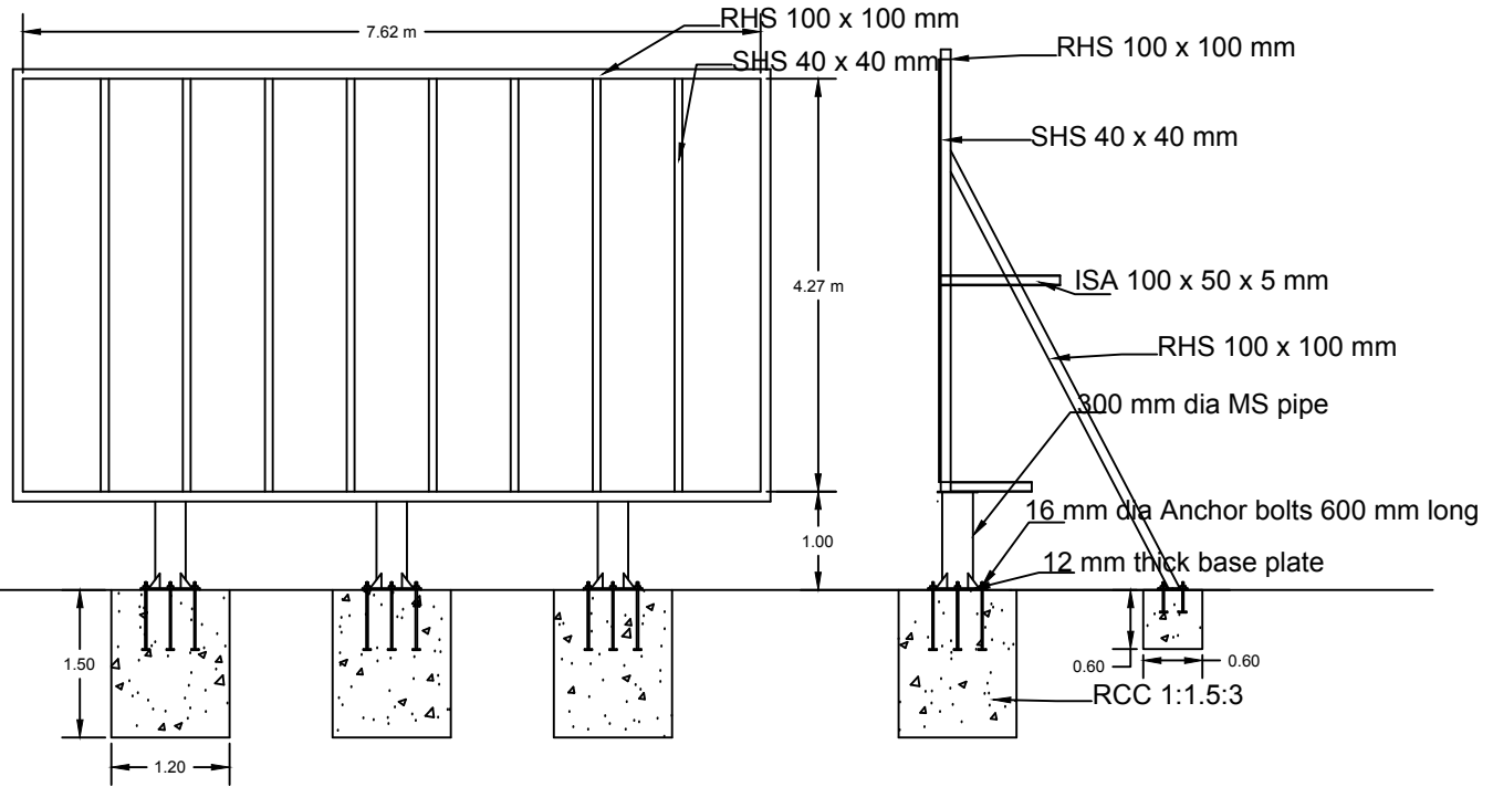
CROSS SECTION
