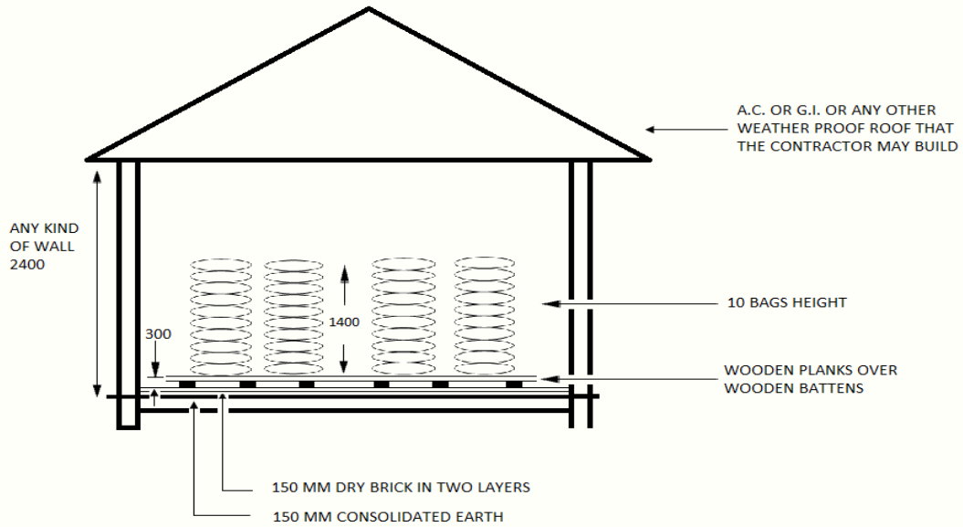
SKETCH OF CEMENT GODOWN
