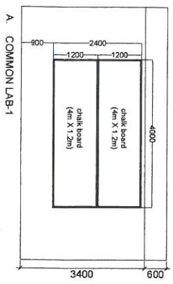
COMMON LAB-1 PLAN
