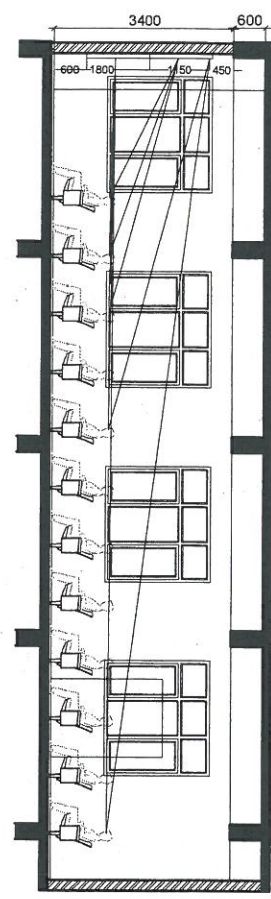
COMMON LAB-1 SECTION
