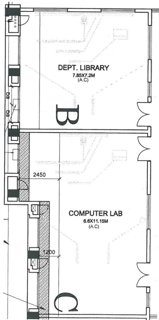
DEPT. LIBRARY PLAN
