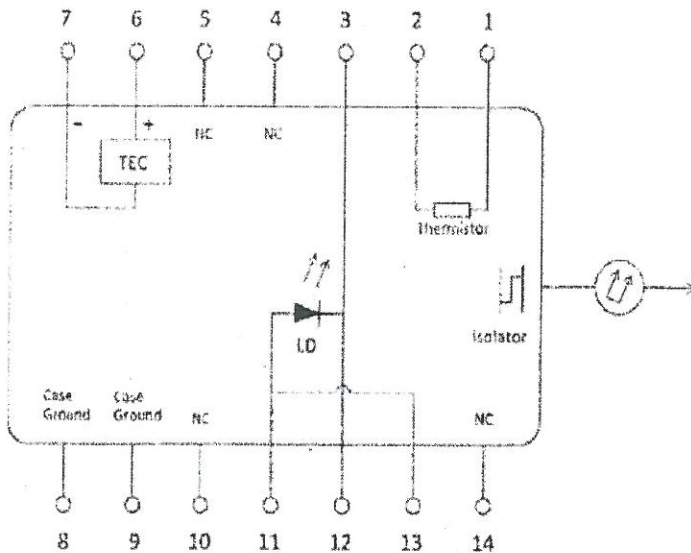
Figure 3: Laser Diode Pin-Out
