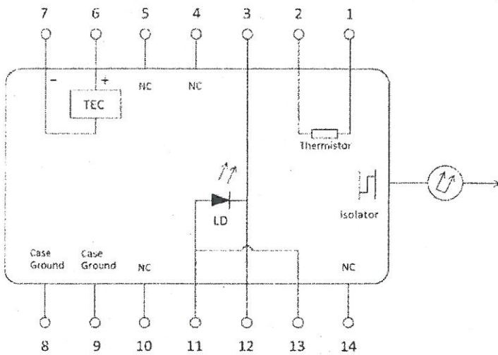
Figure 3: Laser Diode Pin-Out
